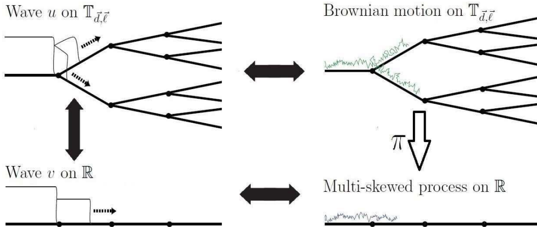
Figure 2: Connection with multi-skewed Brownian motion via projection \pi . [Vertical double-arrow] The top-left part shows the graph of a solution u of (1.1) (the wavefront) on half of a tree, the other half of the tree is symmetric. The wave will propagate to the right (dashed arrows) along all edges of the tree. The bottom left shows an arbitrary semi-infinite branch. Knowing the wave v on it determines the wave u on the entire tree, and vice versa, as described in Lemma 2.3. This is because the travelling waves on any two semi-infinite branches are the same. This equivalence relation is symbolised by the vertical double-arrow. [Horizontal double-arrows] Feynman-Kac formula allows us to write the solutions of reaction diffusion equations in terms of diffusion processes, giving (2.4) in the upper horizontal double-arrow and (2.6) in the lower horizontal double-arrow. [Vertical one-sided arrow] On the right, \pi is the projection that maps the Brownian motion on the tree \mathbb{T}_{d,\ell} to a multi-skewed process Y on \mathbb{R} .
