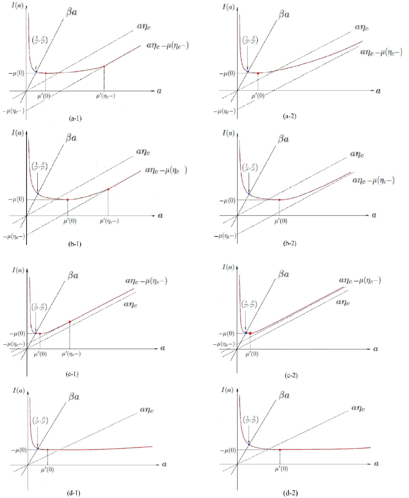
Figure 3: Graph of the function I(a) that exhausts all 8 different cases. The constant- (d, \ell) tree falls into Case (c-2).
