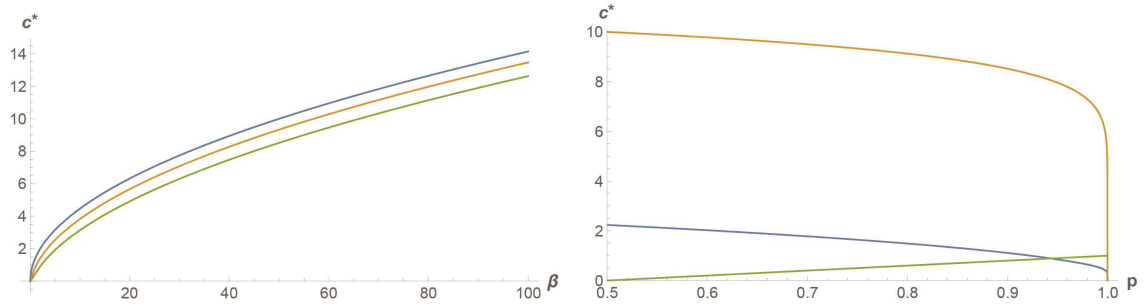
Figure 4: [Left panel] Asymptotic speed c^* versus reaction rate \beta for the constant- (d, \ell) tree. Top curve (blue) is for \mathbb{R} , i.e. d = 2 , so it is exactly \sqrt{2\beta} ; Middle curve (orange) is for (d, \ell) = (4, 1) ; Bottom curve (green) is for (d, \ell) = (10, 1) . Hence the speed decreases as d increases. [Right panel] c^* versus p = \frac{d-1}{d} . Top curve (orange) is for \beta = 50 ; Middle curve (blue) is for \beta = 2.5 ; Bottom curve (green) is the “critical curve” p \mapsto c^*(\beta_c(p), p) .
