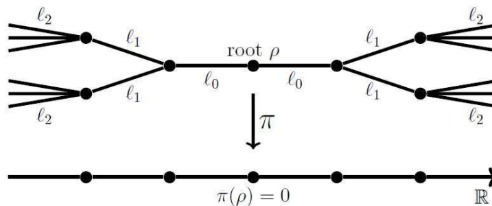
Figure 1: Symmetric \vec{d} -regular tree with branch lengths \vec{\ell} , denoted by \mathbb{T}_{\vec{d}, \vec{\ell}} , with d_0 = 2 , d_1 = 3 and d_2 = 4 . The projection \pi : \mathbb{T}_{\vec{d}, \vec{\ell}} \rightarrow \mathbb{R} maps the root \rho to 0 and (y, k) to y . Let (B_t)_{t \geq 0} be a Brownian motion on \mathbb{T}_{\vec{d}, \vec{\ell}} and define Y_t = \pi(B_t) . Then the projected process Y = (Y_t)_{t \geq 0} is a multi-skewed Brownian motion with skewness (see Definition 5) 2/3 at \ell_0 and skewness 1/3 at -\ell_0 .
